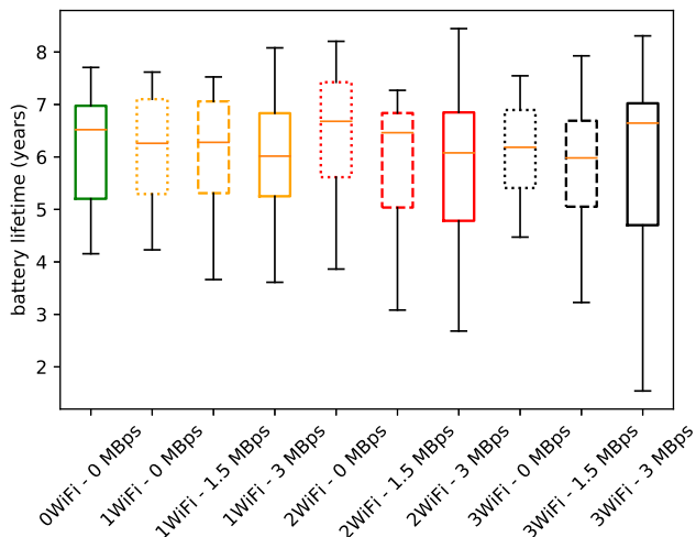
Figure 6: Battery lifetime distribution of all motes. Whiskers show the min/max lifetime, the box the standard deviation around the average lifetime. Battery lifetime for all levels is between 6 and 7 years, and while the impact of WiFi interference is visible, it is minimal.
