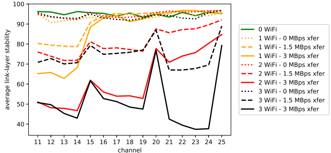
Figure 3: Plotting the link stability as a function of channel clearly shows the frequency band each WiFi router interferes with. We also see that, the worst case WiFi interference is far heavier than what is typically seen in a office environment [13].
