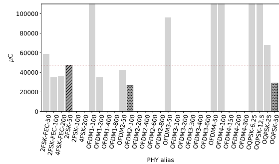
(f) Average electric charge consumption per packet of 2047 B. OFDM2-100 and OQPSK-50 are the less electric charge-hungry radio setting, consuming 26.8 mC and 29.1 mC respectively while 2FSK-50 consumes almost the double, 47.5 mC.
