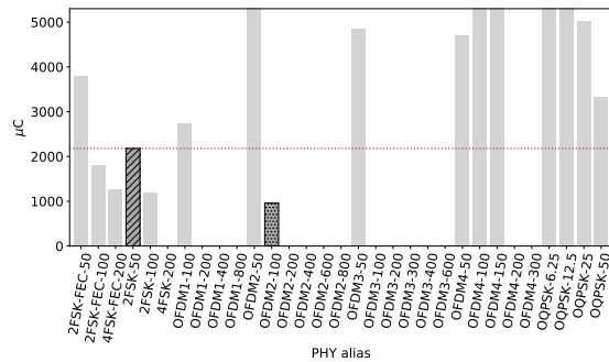
(e) Average electric charge consumption per packet of 127 B. OFDM2-100 consumes the less electric charge, 964 μC while 2FSK-50 consumes 2178 μC.
