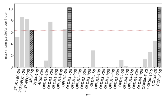
(d) Maximum amount of 2047 B packets that can be correctly sent within an hour. OFDM2-100 and OQPSK-50 can send up to 10 packets, while the reference 2FSK-50 just 6 packets.
