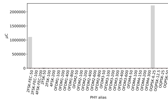
(f) Average electric charge consumed per packet of 2047 B transmitted. In average, it takes more than 1 C per packet using 2FSK-FEC-50 and more than 2 C if OQPSK-6.25 is used.
