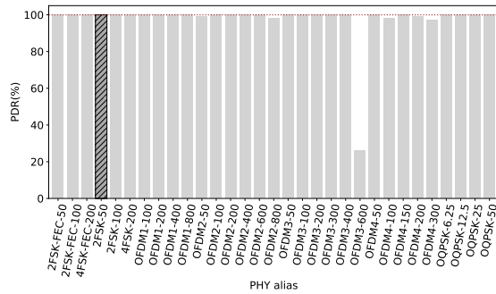
(a) PDR of all radio settings at 420 m from TX with packets of 127 B. Except from OFDM3-600, all radio settings have a PDR close to 100 %.
