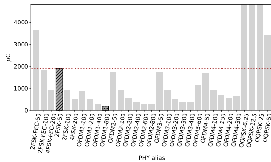
(e) Average electric charge consumed per packet of 127 B sent. OFDM1-800 is the less consuming radio setting, with 184 \mu\text{C} per packet whilst 2FSK-50 consumes 1900 \mu\text{C} .
