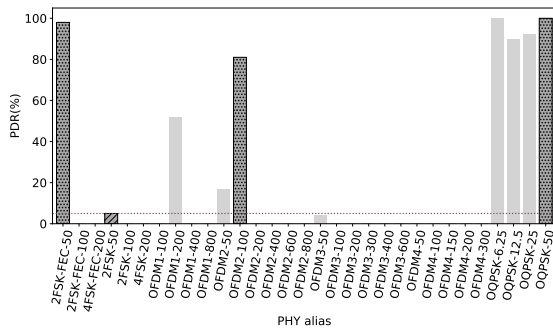
(a) PDR values for all radio settings with short packets. Only 2FSK-FEC-50, OFDM2-100 and all the O-QPSK radio settings have a PDR over 80 %. The reference has a poor PDR, only 5 %.
