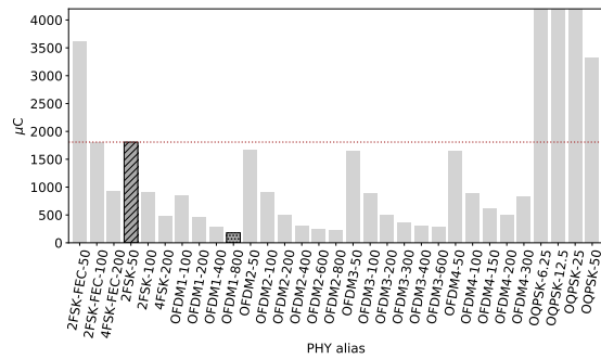
(e) Average electric charge consumed per 127 B packet transmitted. OFDM1-800 is the less power-hungry, with 178 \mu\text{C} consumed, against the 1800 \mu\text{C} needed by 2FSK-50 to transmit the same packet. The rest of the high data rates OFDM PHYs also consume significantly less electric charge than the reference.
