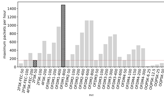
(c) Maximum amount of TX packets of 127 B under the 0.1 % duty cycle regulation. OFDM1-800 can transmit up to 1485 packets, while the reference 158 packets. OFDM2-600 and OFDM2-800 can also transmit more than 1000 short packets.
