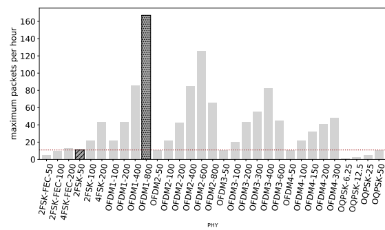
(d) Maximum amount of long packets that can be transmitted per hour. OFDM1-800 can transmit up to 167 packets, more than 10 times the reference with just 11 packets.
