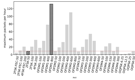
(d) Maximum amount of TX packets of 2047 B under the 0.1 % duty cycle regulation. OFDM1-800 can send up to 132 packets, OFDM2-600 110 packets and the reference just 9 packets.
