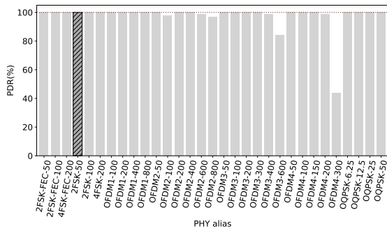
(a) Packets of 127 B. Almost all radio settings with a PDR close to 100 %, including those with the higher data rates.
