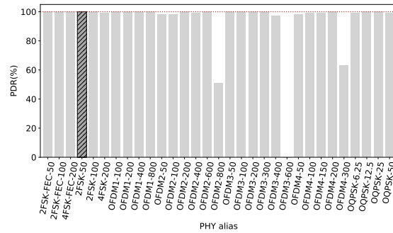
(b) PDR of all radio settings at 420 m from TX with packets of 2047 B. OFDM2-800 and OFDM4-300 do not have PDR values close to 100 %. OFDM3-600 has 0 % PDR.
