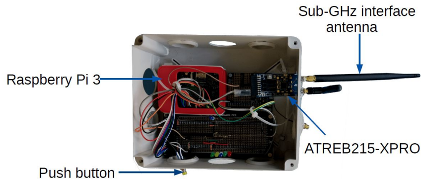
Figure 1. Node used in the range test measurement campaign.
