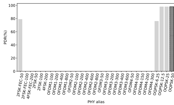
(a) PDR values with packets of 127 B. OQPSK-12.5, OQPSK-25 and OQPSK-50 have 98 % PDR. We see that the most advantageous of that group is OQPSK-50, offering the same reliability with higher data rate.
