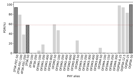
(b) PDR at 700 m from the TX with packets of 2047 B. The reference has 58 % PDR, while 2FSK-FEC-50 94 % PDR and OQPSK-50 100 % PDR.
