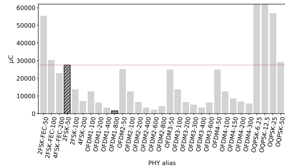
(f) Average electric charge consumed to sent a long packet. Still OFDM1-800 is the less electric charge-consuming, with 1637 \mu\text{C} per packet, whereas the reference consumes 27.5 \text{mC} .
