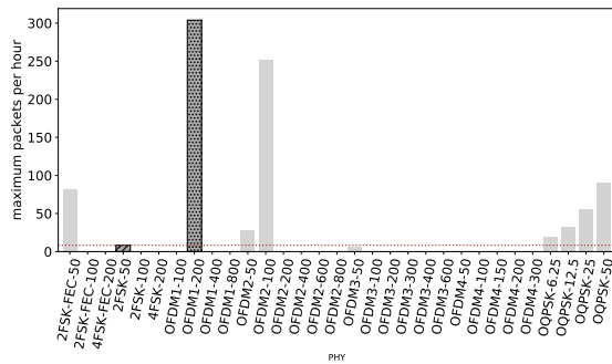
(c) Maximum amount of TXs with short packets under 0.1 % duty cycle. Despite its PDR of 52 %, OFDM1-200 is able to transmit up to 300 short packets. The reference can send just 8 packets.
