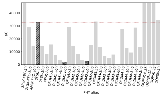
(f) Average electric charge consumed per packet of 2047 B sent. OFDM1-800 and OFDM2-600 are the more electric charge-efficient PHYs, consuming around 2.1 m\text{C} and 2.5 m\text{C} . 2FSK-50 consumes around 33 m\text{C} .
