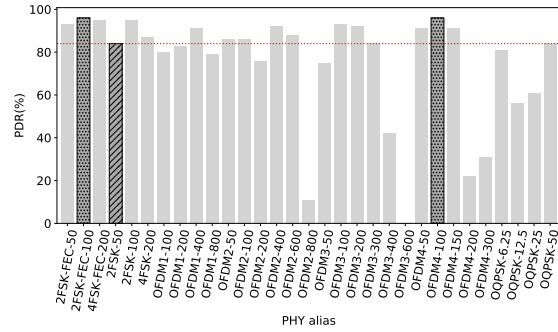
(b) PDR values with 2047 B packets. Overall values are over 50 %, with few OFDM radio settings. Highest values with 2FSK-FEC-100 and OFDM4-100, 95 % PDR and 96 % PDR. Reference value, 84 % PDR.
