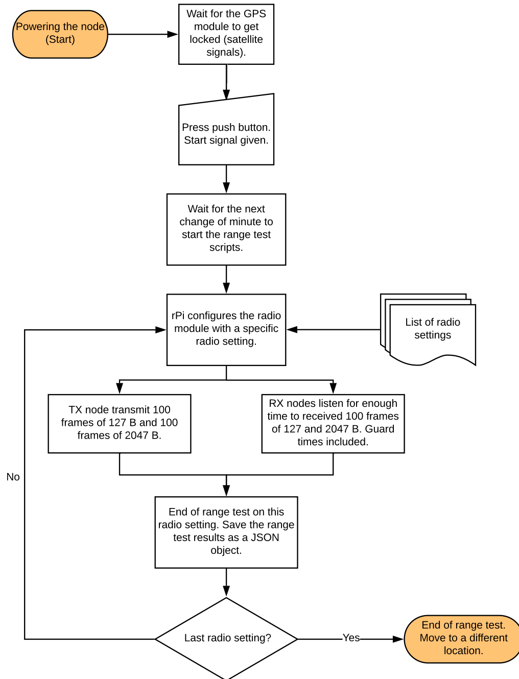
Figure 2. Diagram of the steps followed by each node during an experiment.
