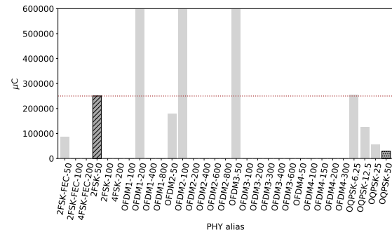
(f) Energy consumed per 127 B packet transmitted. O-QPSK is the less electric charge-consuming radio setting, with 29.5 m\text{C} while the reference consumes 250 m\text{C} .
