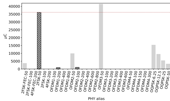
(e) Energy consumed per 127 B packet transmitted. OFDM1-200 and OFDM2-100 are the most electric charge-efficient, consuming 895 \mu\text{C} and 1095 \mu\text{C} respectively. The reference consumes 36 m\text{C} . This is due to its poor PDR.
