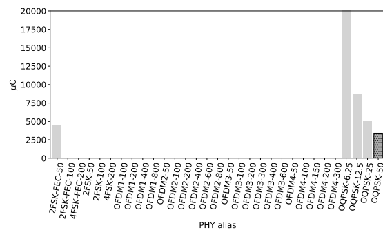
(e) Average electric charge consumed per packet of 127 B transmitted. OQPSK-50 consumes in average, 3.4 mC per packet transmitted.
