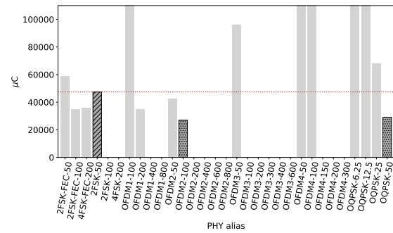
(f) Average electric charge consumption per packet of 2047 B. OFDM2-100 and OQPSK-50 are the less electric charge-hungry radio setting, consuming 26.8 mC and 29.1 mC respectively while 2FSK-50 consumes almost the double, 47.5 mC.
