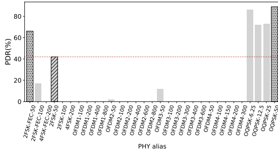
(a) PDR with packets of 127 B. Only data rates up to 50 kbps provide some connectivity, with the exception of O-QPSK-50 whose PDR is above 80 %. We are very close to the maximum length of the radio link. PDR of 2FSK-50 is 42 %.
