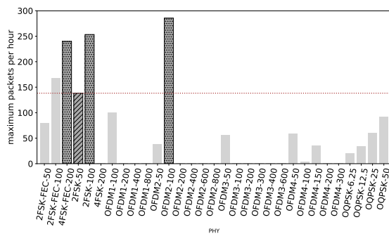
(c) Maximum amount of 127 B packets that can be correctly sent within an hour. 4FSK-FEC-200 and 2FSK-100 can send 239 and 253 short packets. OFDM2-100 can send up to 285 packets, while the reference only 138 packets.
