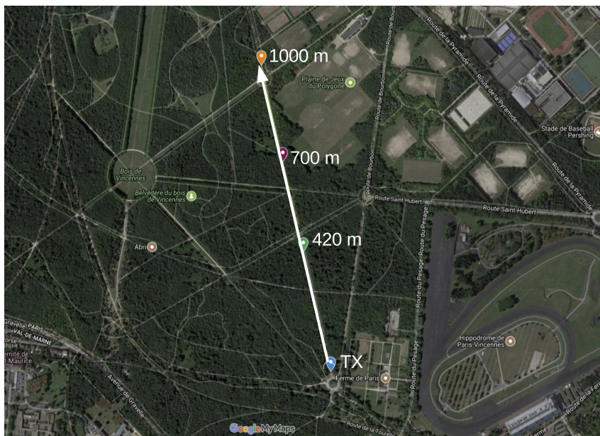
Figure 3. Line of Sight scenario. Distances show where the RX nodes are placed away from the TX node.
