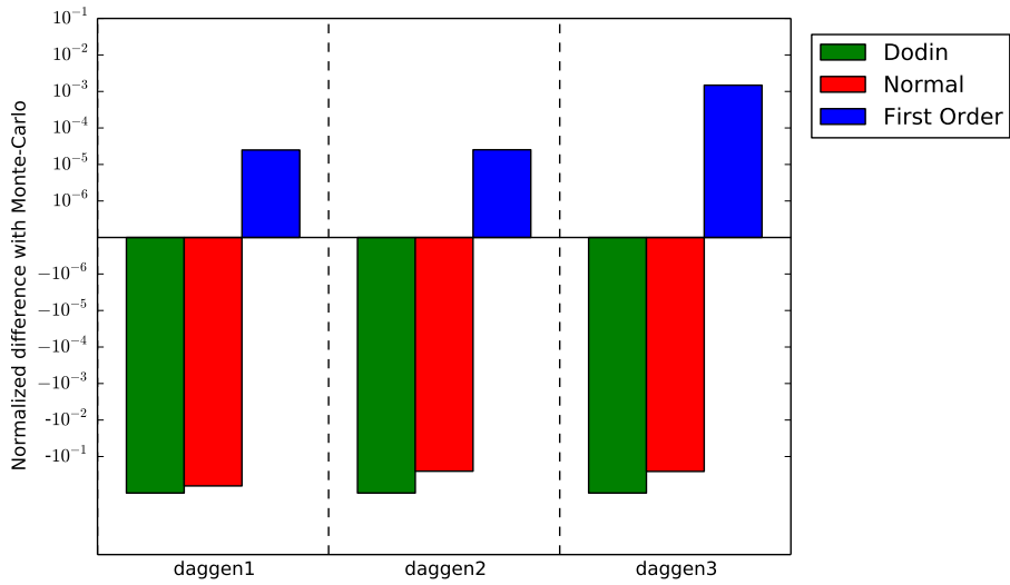
Figure 22: Results on the 3 sets of randomly generated graphs (of size 1000 and various shapes), p_{\text{fail}} = 0.0001
