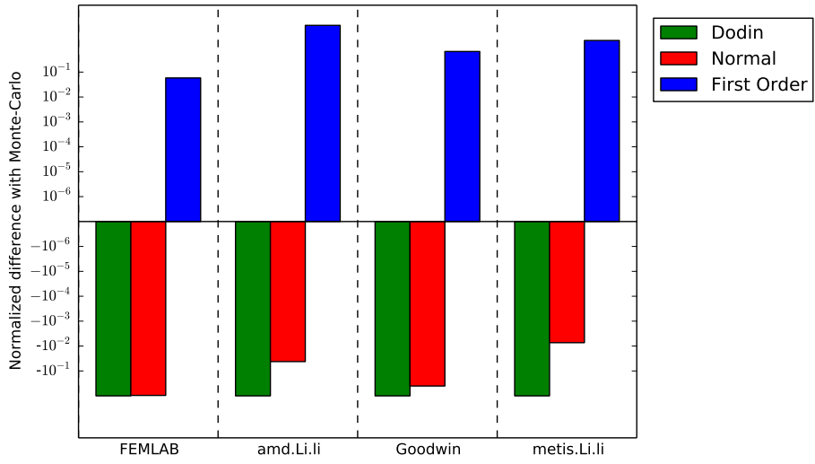
Figure 14: Results on the 4 assembly trees, p_{fail} = 0.01
