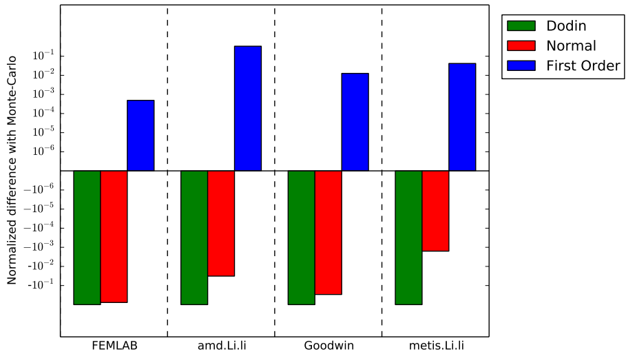
Figure 15: Results on the 4 assembly trees, p_{fail} = 0.001
