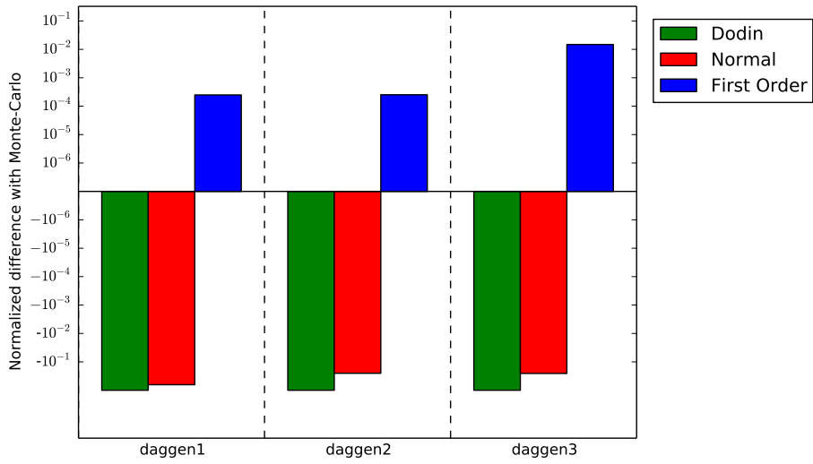
Figure 21: Results on the 3 sets of randomly generated graphs (of size 1000 and various shapes), p_{\text{fail}} = 0.00001
