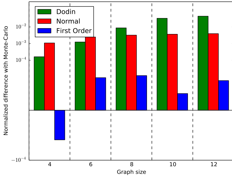
Figure 13: QR ( k = 4, 6, 8, 10, 12 ), p_{\text{fail}} = 0.0001
