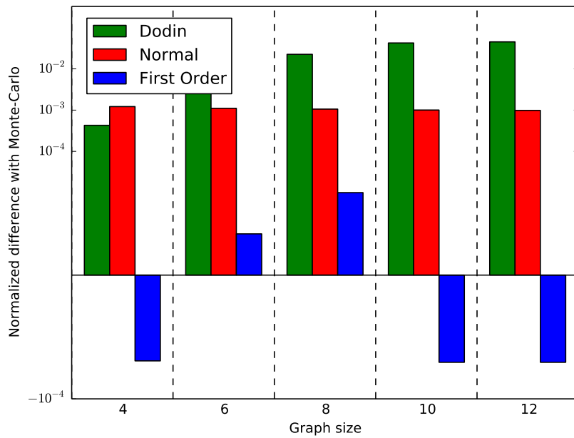
Figure 10: LU ( k = 4, 6, 8, 10, 12 ), p_{\text{fail}} = 0.0001
