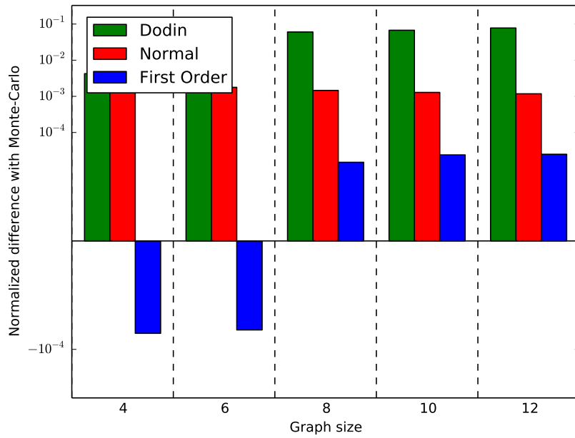
Figure 9: LU ( k = 4, 6, 8, 10, 12 ), p_{\text{fail}} = 0.001
