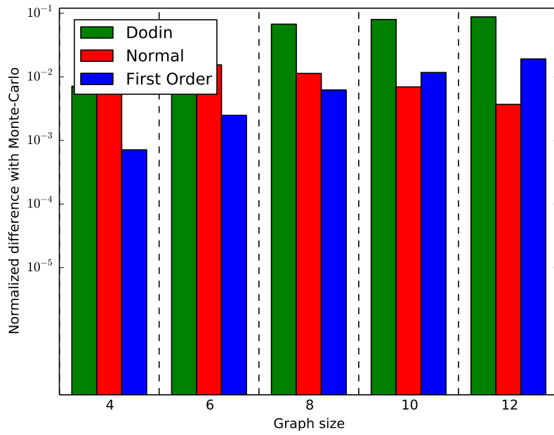
Figure 5: Cholesky ( k = 4, 6, 8, 10, 12 ), p_{\text{fail}} = 0.01
