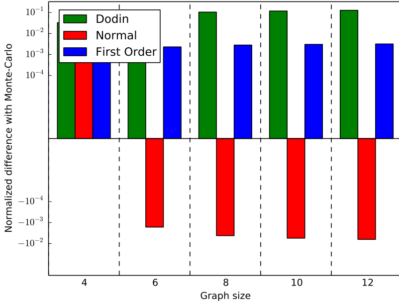
Figure 8: LU ( k = 4, 6, 8, 10, 12 ), p_{\text{fail}} = 0.01
