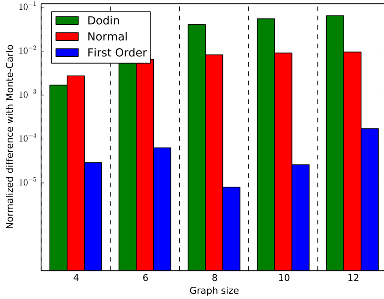
Figure 12: QR ( k = 4, 6, 8, 10, 12 ), p_{\text{fail}} = 0.001
