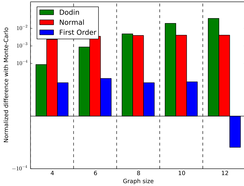
Figure 7: Cholesky ( k = 4, 6, 8, 10, 12 ), p_{\text{fail}} = 0.0001
