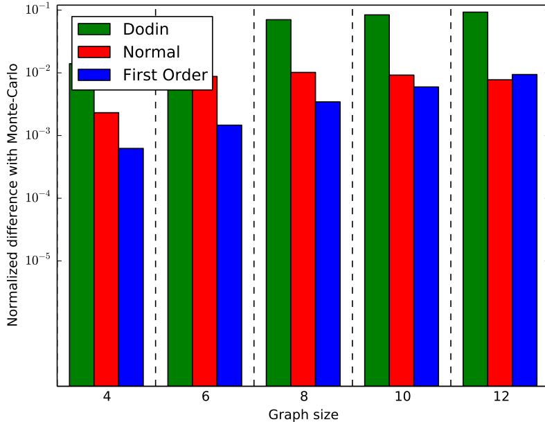
Figure 11: QR ( k = 4, 6, 8, 10, 12 ), p_{\text{fail}} = 0.01
