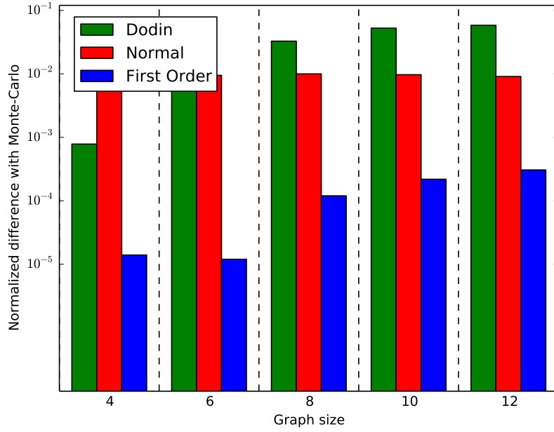
Figure 6: Cholesky ( k = 4, 6, 8, 10, 12 ), p_{\text{fail}} = 0.001
