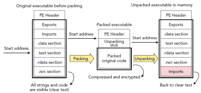
Fig. 3. Life cycle of a program being packed and loaded into memory [18]. The packer takes all the content of the PE file in the highlighted rectangle (not the header) and compresses and encrypts this into a new payload. An unpacking stub is added that is placed at the updated start address of the PE file's execution. The PE header is updated accordingly. The unpacking is performed when the program is executed, by the unpacking stub decrypting and decompressing the original content and recreating the parts of the file shown in the black rectangle. Finally the unpacking stub returns execution to the reinstated start address and the program executes as normal.
