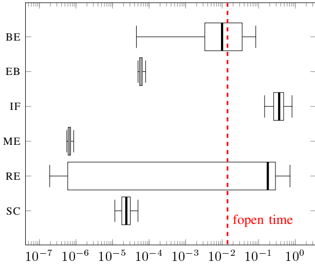
Fig. 4. Feature extraction costs for the feature categories. The dotted red fopen time line represents the empirically-calculated average time for opening the binary before extracting any feature, i.e. 14ms. Extraction cost of the EB, ME, and SC categories is negligible. Extraction cost of the BE and RE categories varies widely according to the size of the file, which sections are present, and whether it is stripped of its debug information and resources. Extraction cost of the IF category is consistently high.
