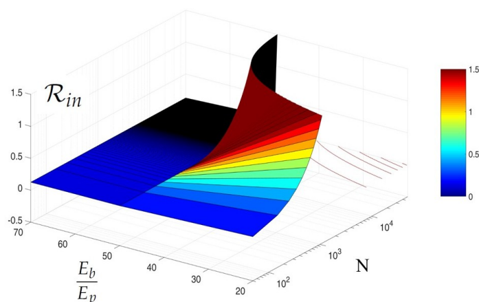
Figure 5. \mathcal{R}_{in} versus E_b/E_p, N , L = 8 , \rho_{CS} = 0.25 , \rho_{enc} = 0.25 .
