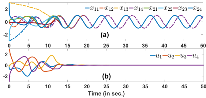
Figure 1. The results of simulation of (11), (26) for N = 4 . a) Evolution of the oscillator states; Bottom) Control signals.
