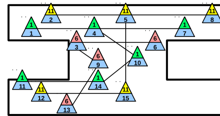
Figure 2: WLAN topology at one floor in our university. The upper number corresponds to the used channel and the lower number corresponds to the AP number.
