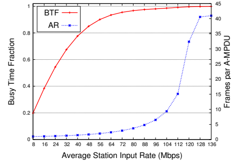
Figure 1: BTF and AR (Aggregation Rate) as function of the input rate.
