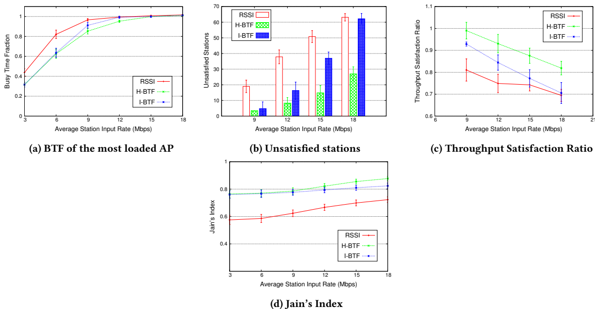
Figure 4: Results for the random topology with UDP flows.
