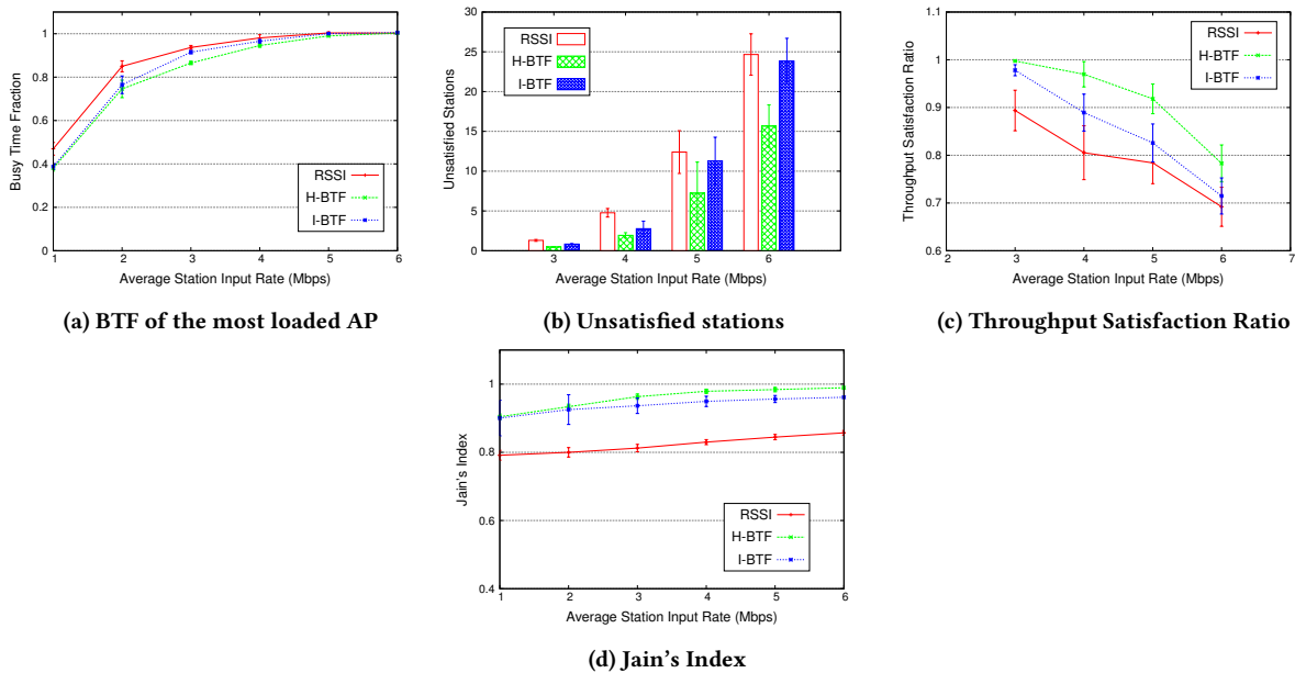
Figure 3: Results for the ENS topology with UDP flows.
