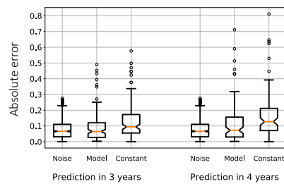
(a) ADAS-Cog
