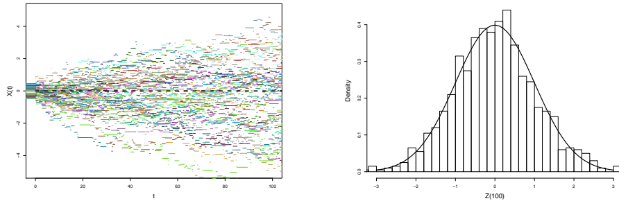
Figure 2: Left: 40 trajectories of X (one color per trajectory) with the parameters defined in (10) with a = 1.01 , b = 1 , q = 1 but Q(d\theta, dy) = \delta_{-1}(d\theta) \otimes \mathbf{1}_{[-1/2, 1/2]}(y)dy and initial condition u^0(\theta, dx) = \mathbf{1}_{[-1/2, 1/2]}(x)dx (uniform law on [-1/2, 1/2] ). The dashed line has slope \mathbf{K} = 0 . Right: distribution of Z(100) = \sqrt{100} \frac{X(100)/100 - K}{\sqrt{\mathbf{Q}}} ( \sqrt{\mathbf{Q}} \simeq 0.20 ), obtained from 1000 trajectories, compared to the density of the normal law.
