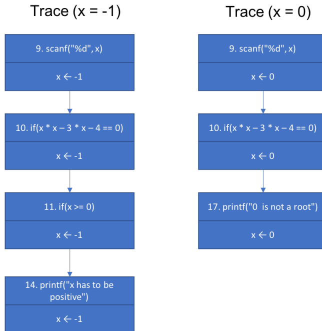
Fig. 9. Example of concrete traces of trial and error root solution.
