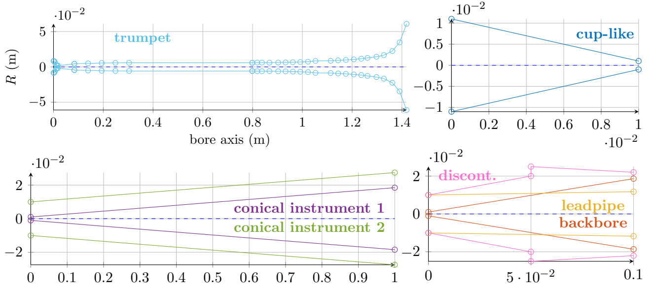
Figure 3: The seven studied bores. Top left : trumpet-like bore. Top right : simple convergent cone of general dimensions similar to a mouthpiece cup. Bottom left : two cones of 1m representative of conical instruments. Bottom right : two cones being qualitatively similar to a mouthpiece backbore and a trumpet leadpipe part, and one arbitrary geometry made of two cones, one divergent, the other convergent, and a clear discontinuity between them. The circles represent the extremities of each part. (colors online)
