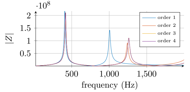
Figure 6: Modulus of the input impedance of a 20 cm cylinder of radius 5 mm computed by the FEM at different orders. (colors online)
