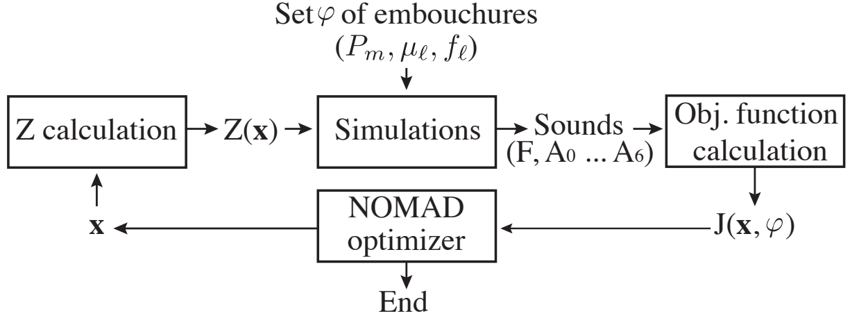
FIG. 3. Flowchart of the optimization process
