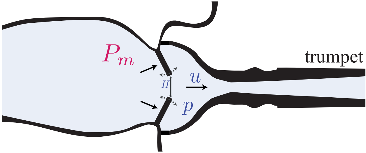
FIG. 2. Representation of the outward striking model of the lips, with the definition of the variables of the physical model: P_m (pressure in the mouth), h (lip aperture), u (volume flow), p (pressure in the mouthpiece)
