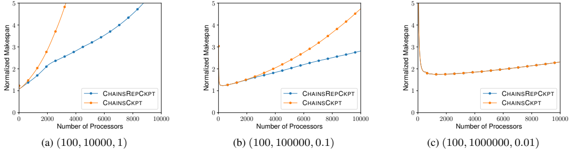
Figure 5: Comparison of the CHAINSCKPT and CHAINSREPCKPT strategies for different numbers of processors, with different model parameter values for the checkpointing cost (a_i, b_i, c_i) .
