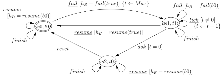
Fig. 5: Open Automaton for the Failure Monitor architecture
