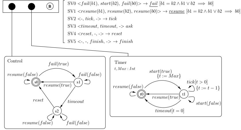
Fig. 2: pNet encoding of the Failure Monitor architecture
