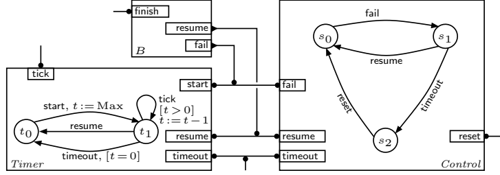
Fig. 1: The BIP specification of the Failure Monitor architecture
