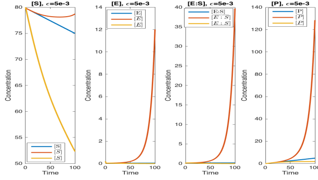
Fig. 1. Bounds on the species' concentration with respect to simulation time, with \epsilon = 5 \cdot 10^{-3} , rate constants k_1 = 0.017, k_{-1} = 0.0017, k_2 = 0.3 , and initial concentrations [S] = 80, [E] = 0.2, [E : S] = 0, [P] = 0 . For each of the 4 species, [\cdot] and [\cdot] denote the lower, respectively upper bounds on its concentration. The depicted results were obtained without using the mass invariants of the original system to constraint the bounds, and as such are suboptimal.
