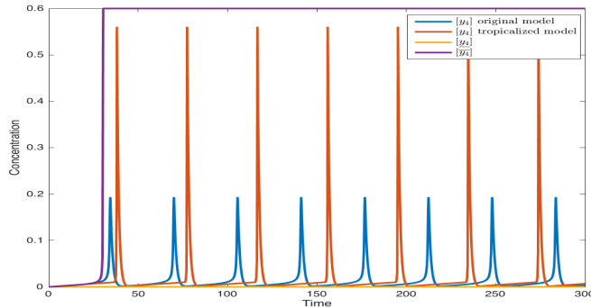
Fig. 5. Estimating the accuracy of the tropicalized Tyson model: bounds on the concentration of [y_4] , with respect to simulation time, for \epsilon = 10^{-3} .
