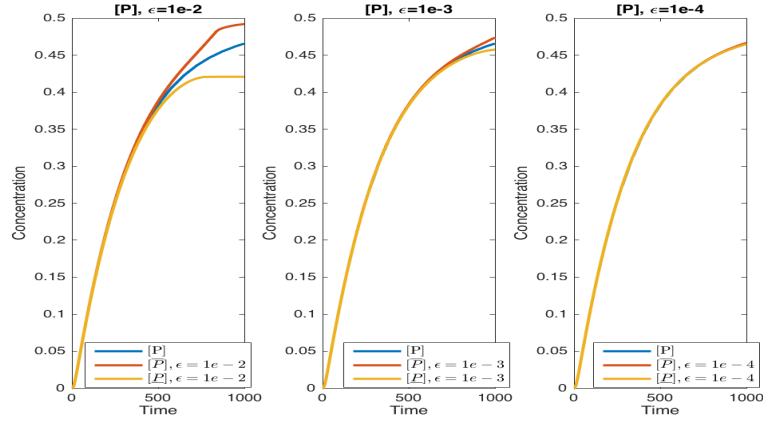
Fig. 3. Bounds on the concentration of P, in the DNA example, obtained by simulating the ODE of tropicalized bounds for different values of the scale separation constant \epsilon , rate constants k_1 = k_2 = k_3 = 0.1, k_{-1} = 0.01, k_{-2} = 0.00001 and initial concentrations [M]_0 = 1, [DNA]_0 = 0.05 .
