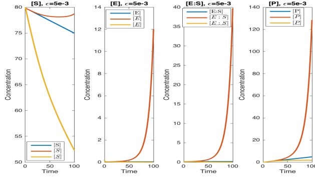
Fig. 1. Bounds on the species' concentration with respect to simulation time, with \epsilon = 5 \cdot 10^{-3} , rate constants k_1 = 0.017, k_{-1} = 0.0017, k_2 = 0.3 , and initial concentrations [S] = 80, [E] = 0.2, [E : S] = 0, [P] = 0 . For each of the 4 species, [\cdot] and [\cdot] denote the lower, respectively upper bounds on its concentration. The depicted results were obtained without using the mass invariants of the original system to constraint the bounds, and as such are suboptimal.
