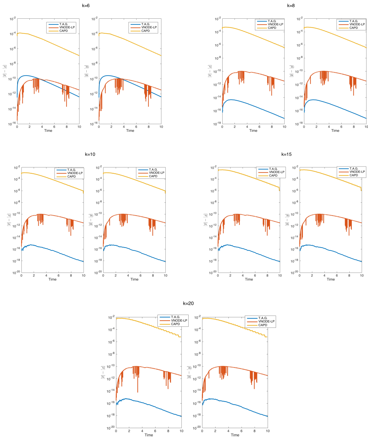
Fig. 6. Comparison of our method - which we denote by "T.A.G."- with existing ODE enclosure methods CAPD and VNODE-LP. For different values of the Taylor expansion order k , used to derive bounds on the system in Example 5.1, our method ultimately out-performs both CAPD and VNODE-LP, in terms of accuracy; for k = 6 , our method is initially outperformed by VNODE-LP on the studied example, but ultimately proves to be more efficient, for the time frame t > 4 . The exponent on the y-axis is an indicator of the decimal precision of the methods (i.e. a value of 10^{-15} means that the first 15 decimals of the computed lower and upper bounds are identical). We also note that both CAPD and VNODE-LP only allow values of k > 4 .
