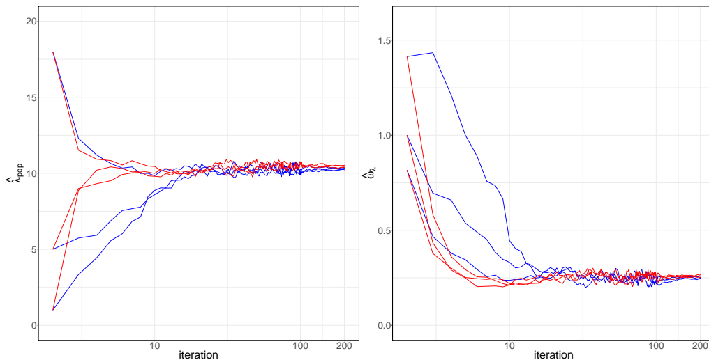
Figure 11: Population parameter estimation in time-to-event-data models: convergence of the sequences of estimates (\hat{\lambda}_{\text{pop},k}, 1 \leq k \leq 200) and (\hat{\omega}_{\lambda,k}, 1 \leq k \leq 200) obtained with SAEM and three different initial values using the reference MH algorithm (blue) and the f-SAEM (red).
