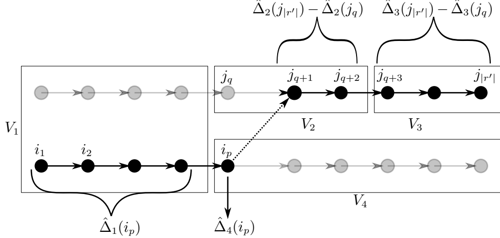
Figure 1 Illustration of r'' and \hat{d}(r'' \cap V_k) for k \in \{1, 2, 3, 4\} . On that example, \hat{\Delta}_2(i_p) = \hat{\Delta}_3(i_p) = \hat{\Delta}_4(j_q) = \hat{\Delta}_4(j_{|r'|}) = 0 while \hat{\Delta}_1(j_q) = \hat{\Delta}_1(j_{|r'|}) , so \hat{d}(r'' \cap V_1) = \hat{\Delta}_1(i_p) , \hat{d}(r'' \cap V_2) = \hat{\Delta}_2(j_{|r'|}) - \hat{\Delta}_2(j_q) , \hat{d}(r'' \cap V_3) = \hat{\Delta}_3(j_{|r'|}) - \hat{\Delta}_3(j_q) , and \hat{d}(r'' \cap V_4) = \hat{\Delta}_4(i_p) .
