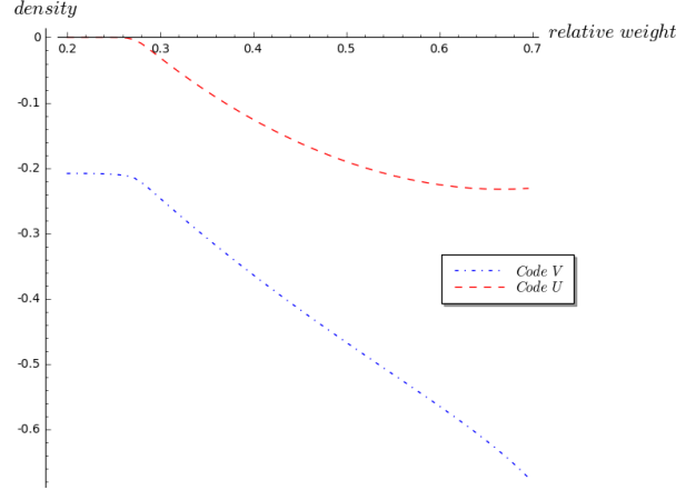
Fig. 11. \alpha_u(w/n) and \alpha_v(w/n) against x \triangleq \frac{w}{n} .
