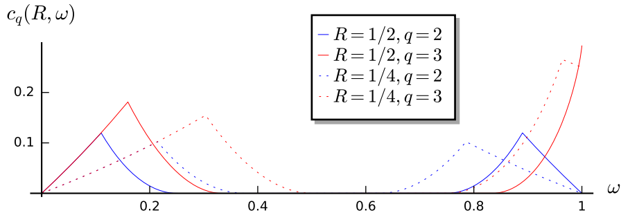
Fig. 9. Asymptotic exponent of Prange's algorithm for code rate R \in \{1/4, 1/2\} and q \in \{2, 3\}
