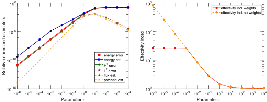
Figure 8: [Section 6.1, \epsilon varies, \kappa = 10^2 , m = 3 ] Relative error and estimate together with their components (left), effectivity indices for weighted and unweighted error estimators (right). Uniform 16 \times 16 \times 2 mesh, polynomial degree p = 1 .
