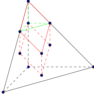
Figure 9: Subdivision of the unit simplex used in the proof of Theorem A.2. The unit simplex is shown for d = 3 , along with its sub-simplex K_\dagger (edges shown in green) and sub-parallelepiped Q_\dagger (edges shown in red).
