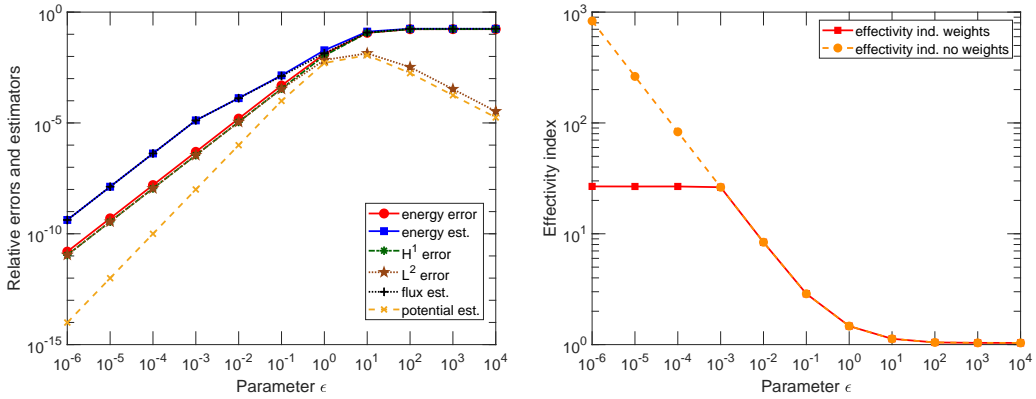
Figure 8: [Section 6.2, \epsilon varies, \kappa = 10^2 , m = 3 ] Relative error and estimate together with their components (left), effectivity indices for weighted and unweighted error estimators (right). Uniform 16 \times 16 \times 2 mesh, polynomial degree p = 1 .
