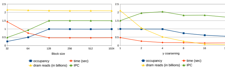
Fig. 1. Grid reshaping
