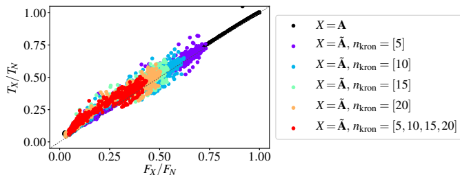
Fig. 5: Normalized number of flops vs. normalized running times for ISTA ( tol = 10^{-5} , \Gamma = 0.5 ). Each point on the graph corresponds to an independent run at a given regularization \lambda/\lambda_{\max} \in [10^{-2}, 1] . Results for the usual GAP Safe test are shown in black and those using its stable version (as in Alg. 1) are shown in colors. The closer the dots lie to the identity line, the better the theoretical speedups are met in practice.
