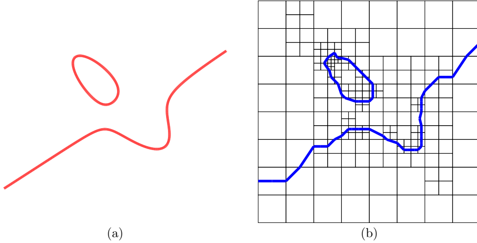
Figure 1: (a) The real curve given by the zeros of f = 3y^3 + 3xy^2 - 2x^3 - 3y^2 + xy + 3x^2 - 3y + 3x + 2 . (b) The approximation produced by the PV algorithm (Plantinga and Vegter, 2004) as well as the regions constructed by the algorithm.
