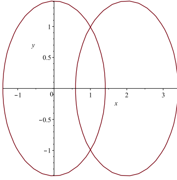
Fig. 2 Intersection between two circles
