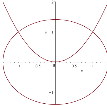
Fig. 1 Intersection between a circle and a parabola
