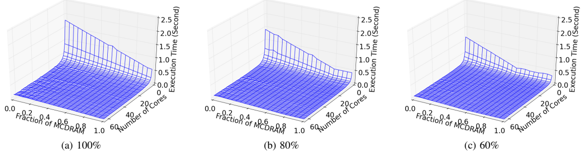
Figure 2. Profiles of the triad application in Stream benchmark when its memory footprint occupies 100%, 80% and 60% of the entire fast memory.
