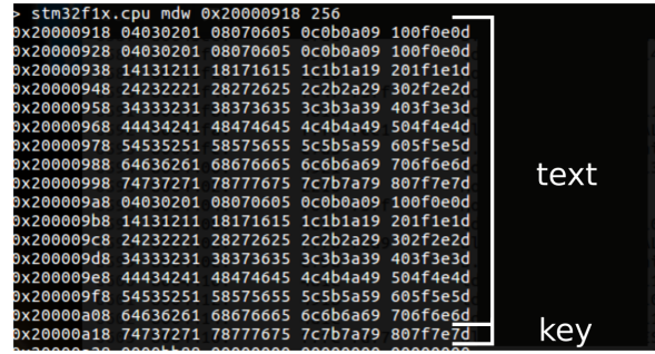
Figure 1: Memory observed with OpenOCD after a successful fault injection. The correct text address is 0x20000918, the first 4 words are correct, resulting from a previous unfaulted execution. The key address is 0x20000a18.
