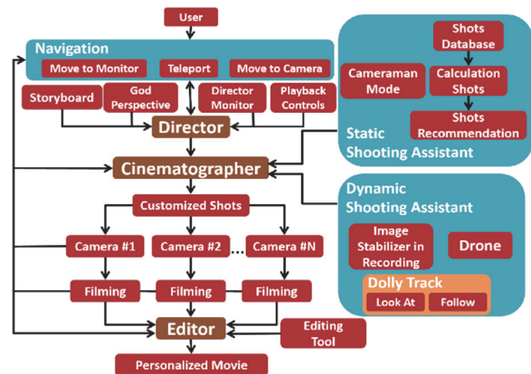
Figure 1: System workflow
