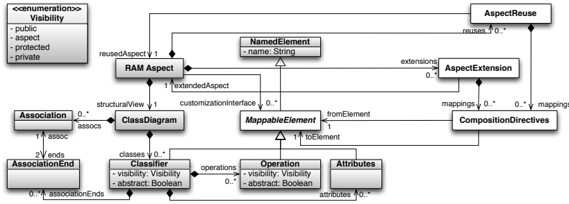
Fig. 4 Parts of the Class Diagram Metamodel of the RAM Modelling Approach
