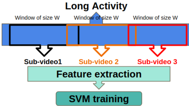
Fig. 1. The training process for our classifier. First, training videos are divided into windows of size W frames, representing activity sub-parts. Then the features are generated for these windows and the training is done with SVM
