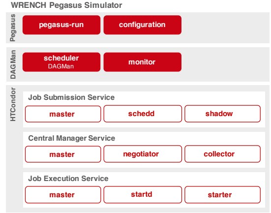
Fig. 3: Overview of the WRENCH Pegasus simulation components, including components for DAGMan and HTCondor frameworks. Red boxes denote Pegasus services developed with WRENCH’s Developer API, and white boxes denote WRENCH reused components.
