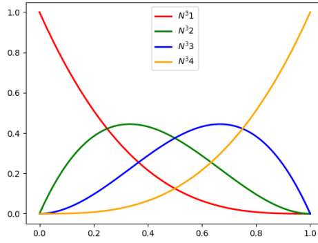
Figure 27: b-spline basis function associated to the knot vector S = [0, 0, 0, 0, 1, 1, 1, 1]
