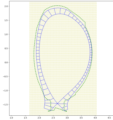
Figure 32: A regular grid of the SOL region.
