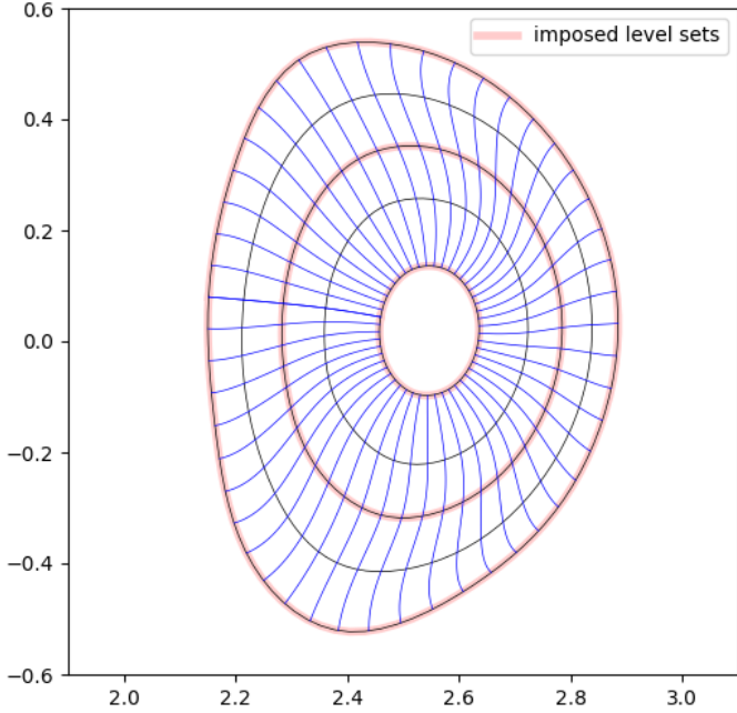
Figure 26: Tensor product surface of a patch enclosed by two level sets.
