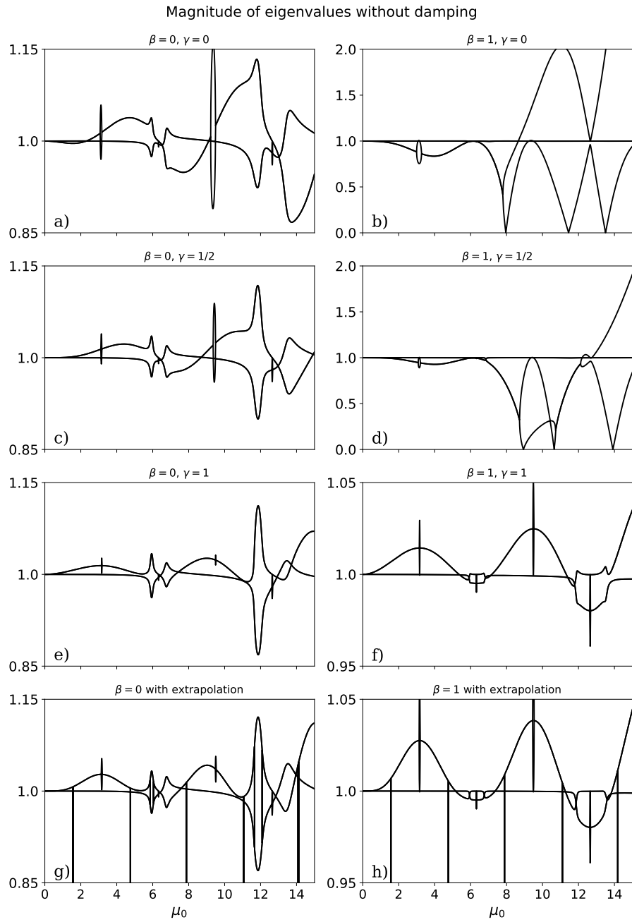
Figure 9: Magnitude of eigenvalues for several choices of \beta, \gamma and for N = 10^{-2} (N_{\text{split}} = 20) . Note that the vertical axes differ among the plots.
