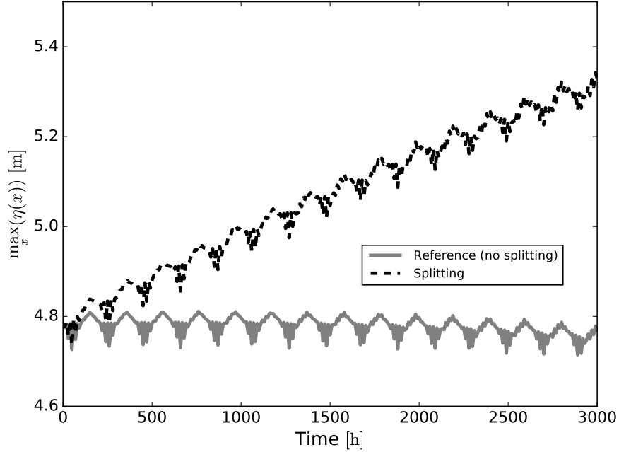
Figure 2: Time evolution of the maximum absolute value of the free surface elevation. Comparison of the numerical solution with (dashed line) and without (plain line) splitting.
