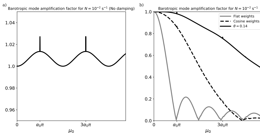
Figure 6: Barotropic mode amplification for N = 10^{-2} , H = 4000 . a) No damping, b) with damping according to different filters (plain line: Flat filter; dashed line: Cosine filter; Thick plain line: FB scheme with \theta = 0.14 ).
