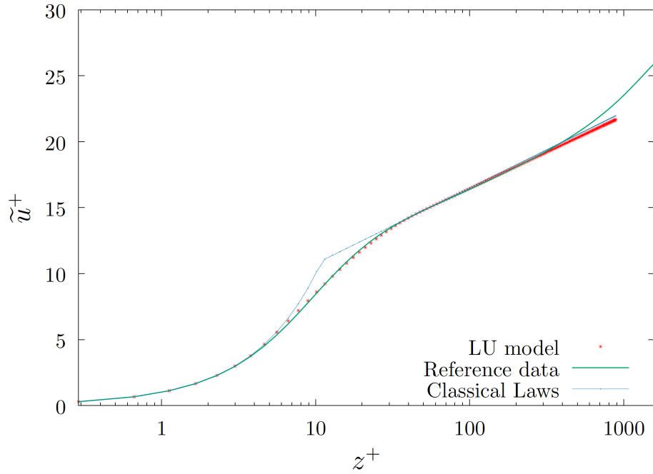
FIG. 3. Velocity profiles for the turbulent boundary layer at Re_\tau = 1709 . The green curve corresponds to the reference data. The blue dot lines show the classic laws (linear then logarithmic) and the red dots corresponds to the profile of the model under location uncertainty.
