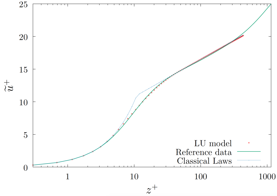
FIG. 1. Velocity profiles for the turbulent boundary layer at Re_\tau = 1306 . The green curve corresponds to the reference data. The blue dot lines show the classic laws (linear then logarithmic) and the red dots corresponds to the profile of the model under location uncertainty.
