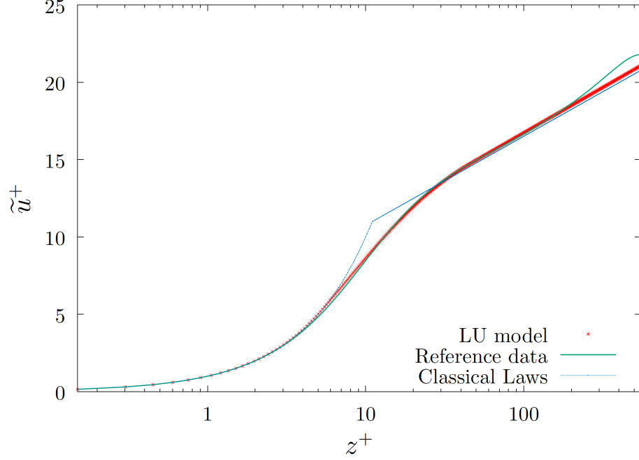
FIG. 7. Velocity profiles for the pipe flow at \text{Re}_\tau = 550 . The green curve corresponds to the reference data. The blue dot lines show the classic laws (linear then logarithmic) and the red dots corresponds to the profile of the model under location uncertainty.
