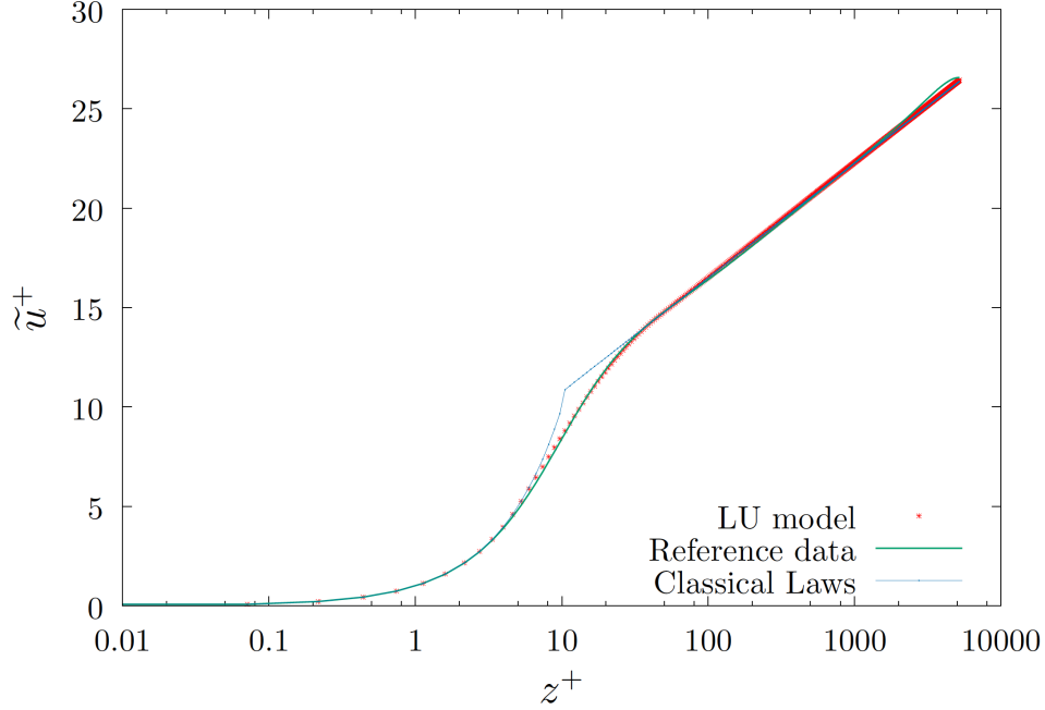
FIG. 9. Mean velocity profiles for the channel flow at \text{Re}_\tau \approx 5200 [? ]. The green curve corresponds to the reference data. The blue dot lines show the classic laws (linear then logarithmic) and the red dots corresponds to the profile of the model under location uncertainty.
