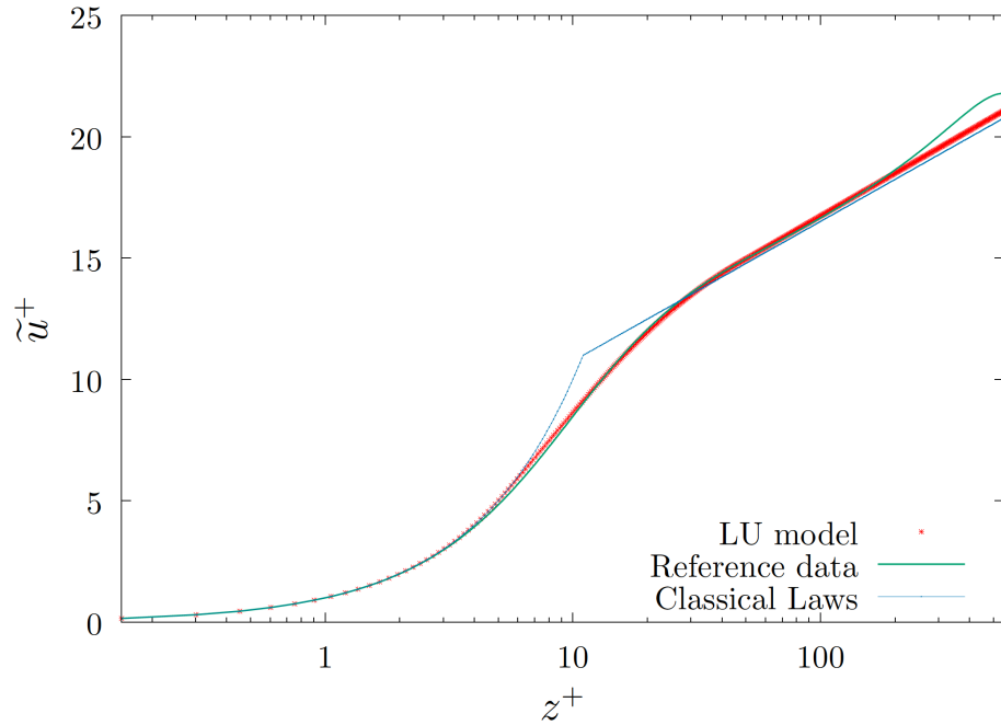
FIG. 7. Velocity profiles for the pipe flow at Re_\tau = 550 . The green curve corresponds to the reference data. The blue dot lines show the classic laws (linear then logarithmic) and the red dots corresponds to the profile of the model under location uncertainty.
