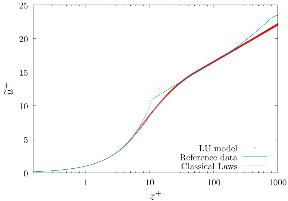
FIG. 7. Velocity profiles for the pipe flow at Re_\tau = 550 . The green curve corresponds to the reference data. The blue dot lines show the classic laws (linear then logarithmic) and the red dots corresponds to the profile of the model under location uncertainty.
