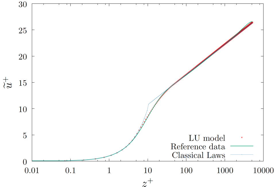
FIG. 9. Mean velocity profiles for the channel flow at Re_\tau \approx 5200 [32]. The green curve corresponds to the reference data. The blue dot lines show the classic laws (linear then logarithmic) and the red dots corresponds to the profile of the model under location uncertainty.
