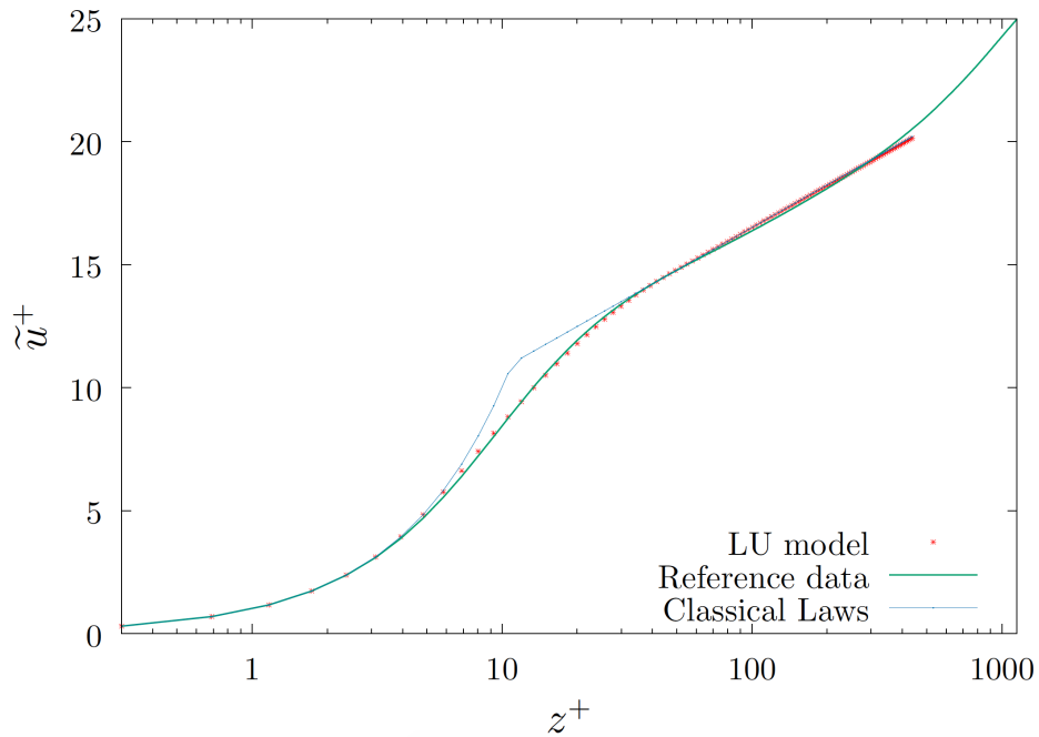
FIG. 1. Velocity profiles for the turbulent boundary layer at \text{Re}_\tau = 1306 . The green curve corresponds to the reference data. The blue dot lines show the classic laws (linear then logarithmic) and the red dots corresponds to the profile of the model under location uncertainty.
