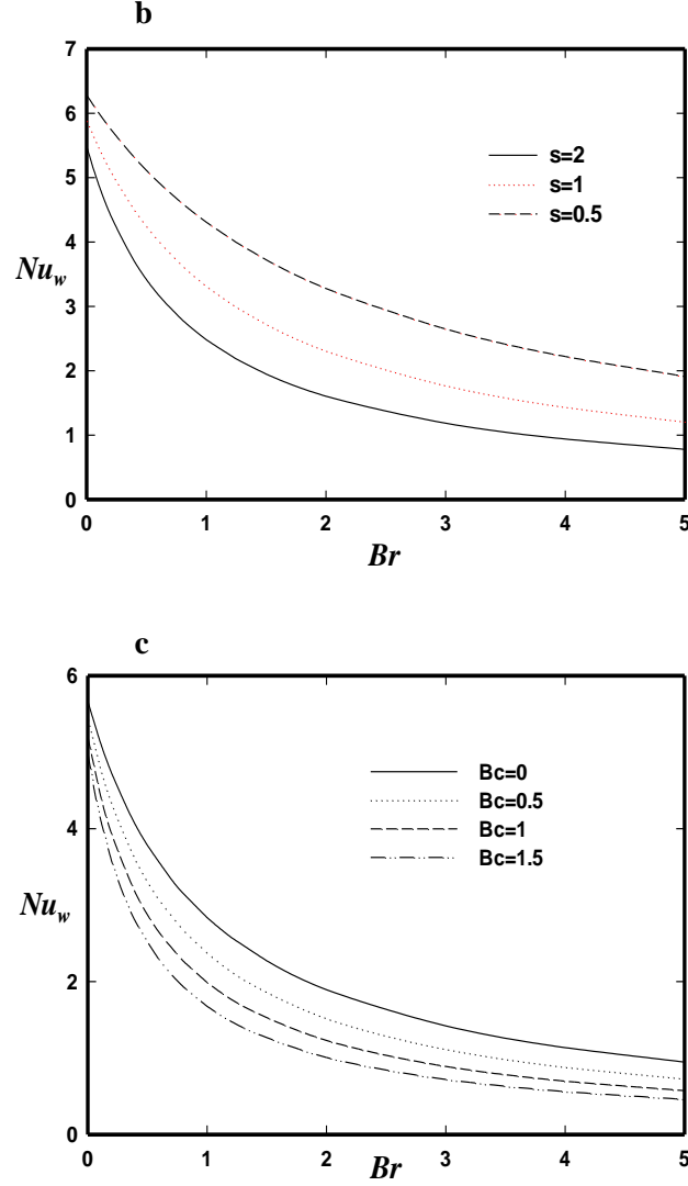
Fig.5. Variation of Nu_w versus Br in the case of fluid heating ( Br>0 ) for \alpha=0.1 , De=1 and a- dimensionless slip number ( B ) at s=1 and Bc=0 b- power law index of slip ( s ) at B=2 and Bc=0.5 c- dimensionless slip critical shear stress number ( Bc ) at B=4 and s=1 .
