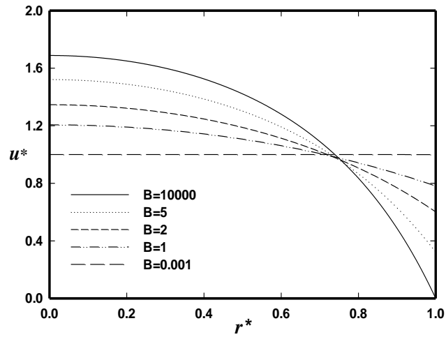
Fig.4. Dimensionless velocity profile with variation of the B for \alpha=0.1 , De = 1 , s = 1 and Bc = 0 .
