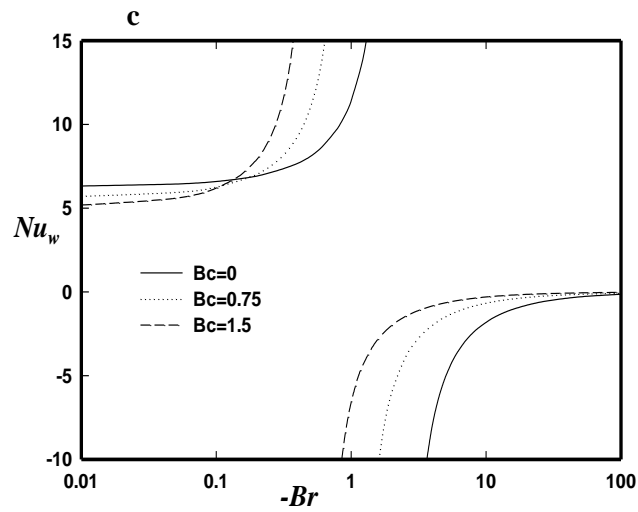
Fig.8. Variation of Nu_w versus Br in the case of fluid cooling ( Br < 0 ) for \alpha=0.1 , De=1 and a- dimensionless slip number ( B ) at s=1 and Bc=0.2 b- power law index of slip ( s ) at B=3 and Bc=0.5 c- dimensionless slip critical shear stress number ( Bc ) at B=2 and s=1 .
