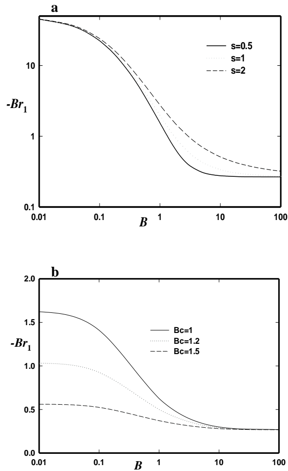
Fig.7. Variation of first critical Brinkman number ( Br_1 ) versus dimensionless slip number ( B ) in the case of fluid cooling ( Br < 0 ) for \alpha=0.1 , De=1 and a- power law index of slip ( s ) at B_c=0.2 b- dimensionless slip critical shear stress number ( B_c ) at s=1 .
