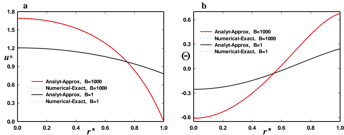
Fig.3- Dimensionless a- velocity profile for \alpha=0.1 , De = 1 , s = 1 and Bc = 0 b- temperature profile for \alpha=0.1 , De = 1 , s = 0.5 and Bc = 0.5 .
