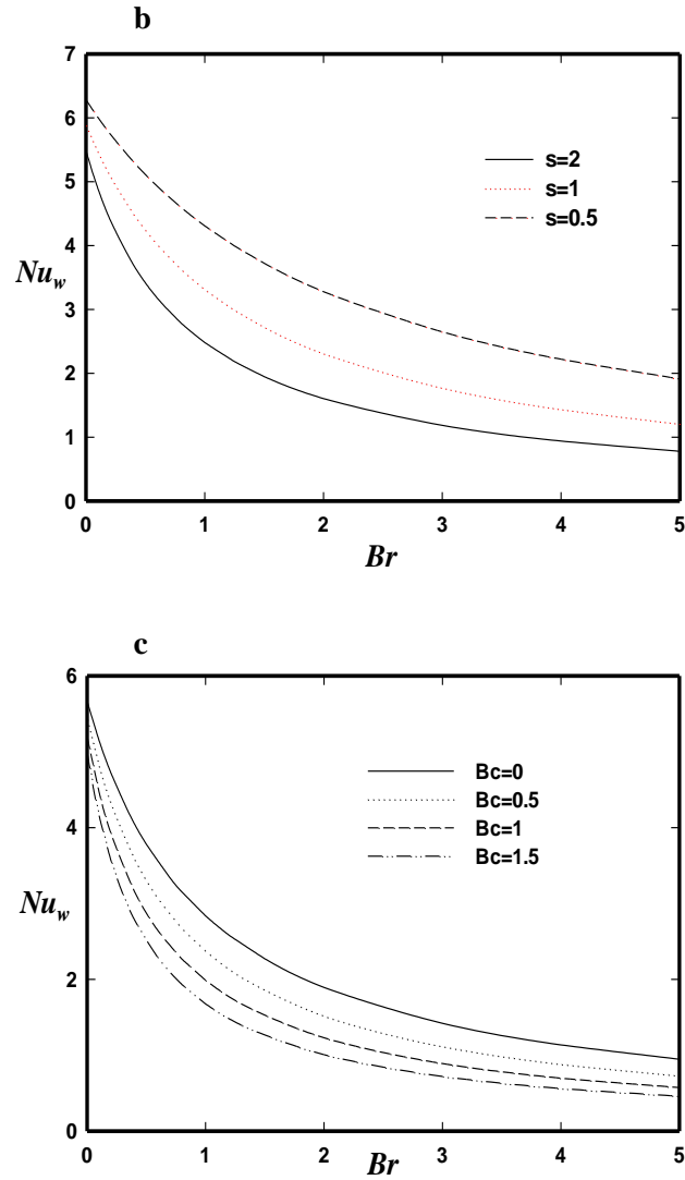
Fig.5. Variation of Nu_w versus Br in the case of fluid heating ( Br > 0 ) for \alpha=0.1 , De=1 and a- dimensionless slip number ( B ) at s=1 and Bc=0 b- power law index of slip ( s ) at B=2 and Bc=0.5 c- dimensionless slip critical shear stress number ( Bc ) at B=4 and s=1 .
