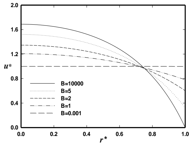
Fig.4. Dimensionless velocity profile with variation of the B for \alpha=0.1 , De = 1 , s = 1 and Bc = 0 .
