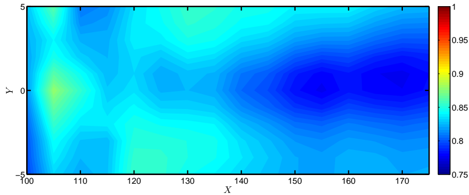
Fig. 7 Correlation map for the actuation transfer function calculated using PSE. A similar behaviour is observed with the empirical model.
