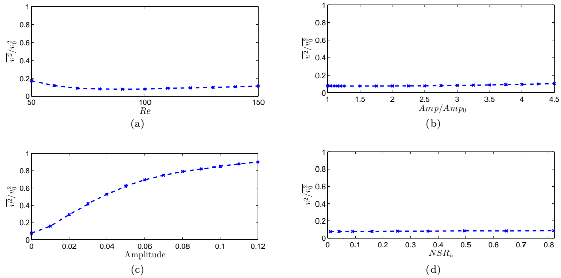
Fig. 16 Robustness evaluation of the inversion controller, MS of the transverse velocity components of the controlled case divided by the corresponding open-loop scenario. (a) Reynolds number variation (control laws were designed for Re = 100 ), (b) Amplitude of the inflow perturbations divided by their nominal value, (c) Amplitude of the perturbations inserted between input and output positions, (d) Noise in the actuation signal (a similar behaviour was observed for the case of measurement noise and will not be shown here, for the sake of brevity.)
