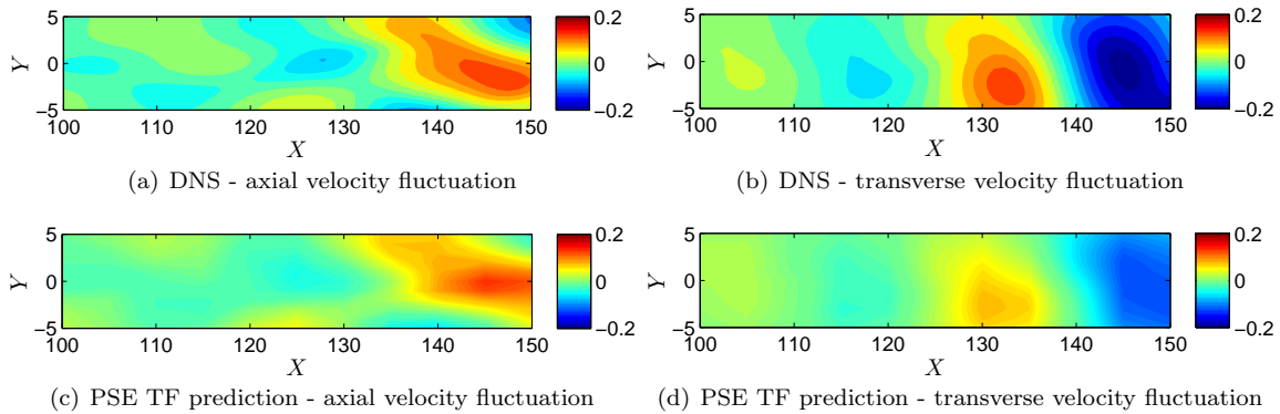
Fig. 5 Results of the direct numerical simulation in comparison to PSE transfer function predictions for axial and transverse velocity fluctuations.
