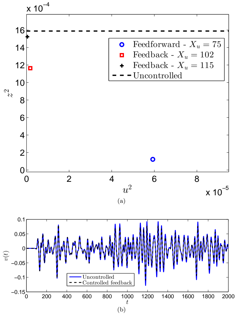
Fig. 21 Results for feedback control compared to corresponding feedforward configuration, actuation and objective are fixed at 100 and 125, respectively, input varies from 75 (feedforward configuration), 102 and 115 (feedback configurations). (a) MS values of the objective and actuation, (b) time series for a feedback configuration, for X_u = 115 , in comparison to the open-loop behaviour.
