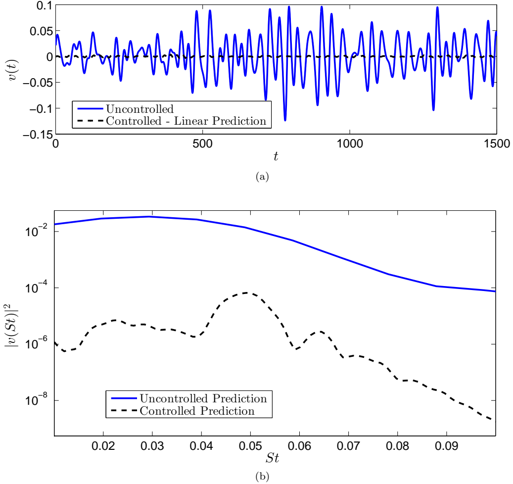
Fig. 11 Closed-loop behaviour for the linearised system using wave-cancellation in the (a) time and (b) frequency-domain.
