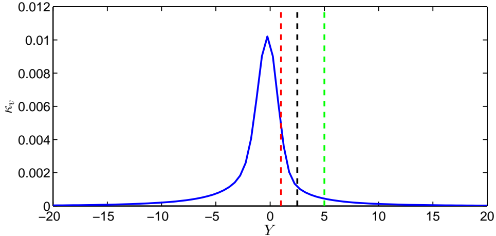
Fig. 17 Sensitivity index for transverse forcing aiming at v , vertical lines indicate other transverse positions that were considered in figure 18, for comparison with the optimal case.
