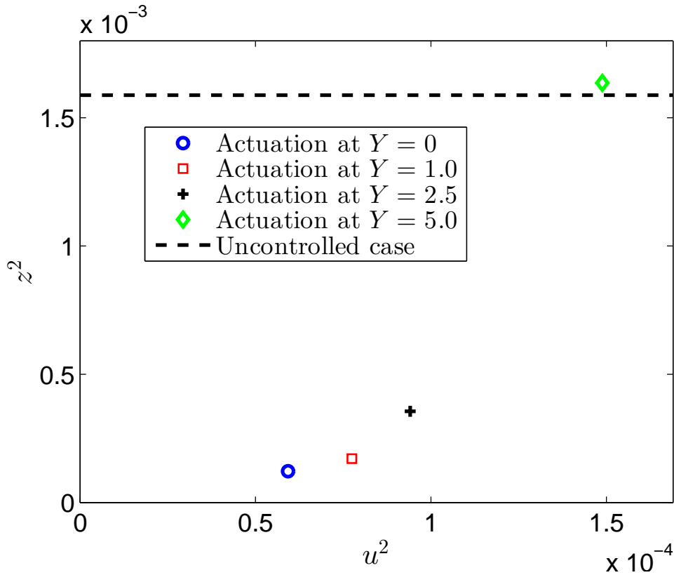
Fig. 18 Comparison of the mean square values for the objective and actuation signals at 4 different transverse positions, at X_u = 100 . The dashed line indicates the MS of the output for the open-loop case
