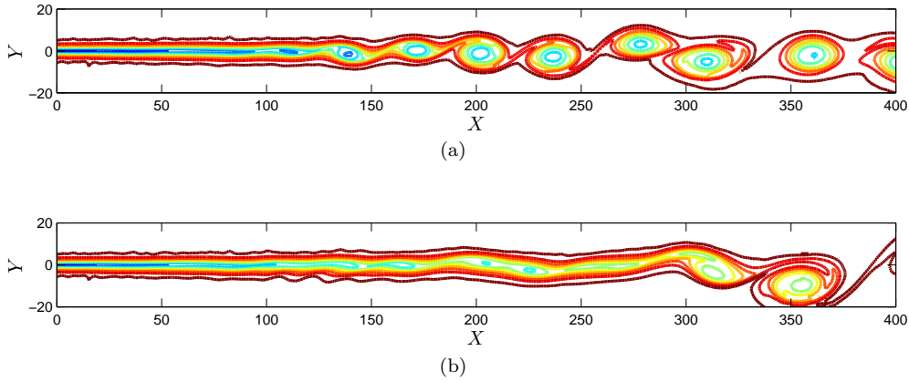
Fig. 15 Comparison of the vorticity fluctuations for the uncontrolled (a) and controlled (b) cases at t = 1200 . The delay in the vortex pairing becomes apparent.
