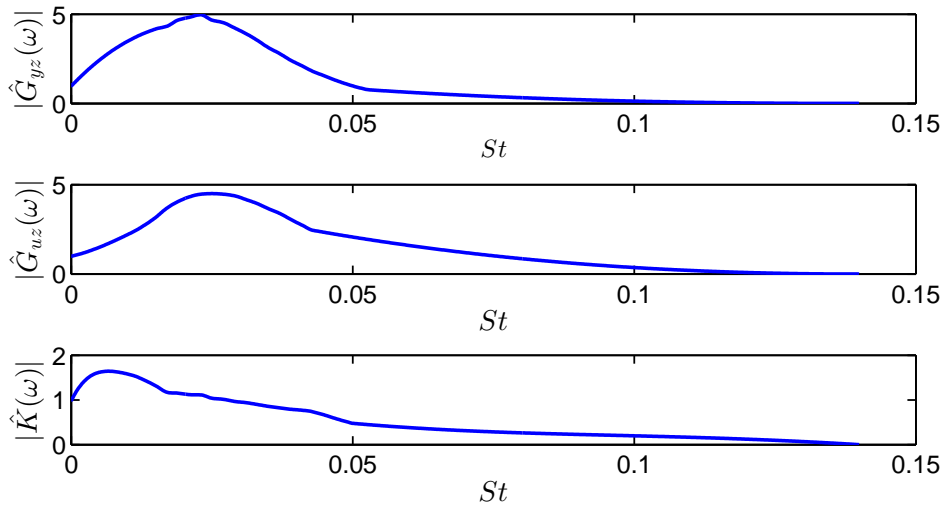
Fig. 10 Resulting actuation transfer functions between estimation, actuation and output and computed gain for compensator. Subscripts y, u, z define input, actuation and output positions, localized at X = 75, 100 and 125 , respectively and at the centerline of the flow, considering the axial velocity fluctuation. The actuation corresponds to a transverse forcing.
