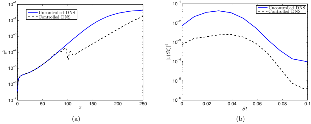
Fig. 14 (a) Mean-squared value for the transverse velocity fluctuation in the centerline of the flow. (b) Power spectral densities of the uncontrolled and controlled non-linear simulations for the transverse velocity fluctuation at the objective position.
