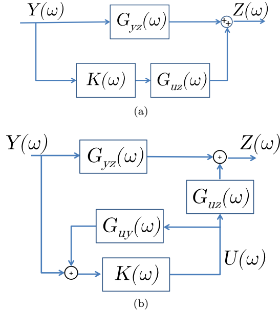
Fig. 8 Block diagram for (a) feedforward and (b) feedback control laws. \hat{G}_{yz} and \hat{G}_{uz} are the estimating and actuation transfer functions between input/acting positions and output, respectively. It should be noted that the branch where the transfer function \hat{G}_{uy} is located is added in the feedback scheme, which accounts for the effect of the actuation into the input sensor. The frequency dependent gain \hat{K}(\omega) is designed separately for each configuration.
