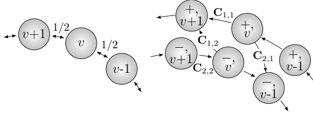
Figure 1: (left) random walk \mathbf{P}_0 on the N -cycle; (right) quantum walk unitary with coin toss \mathbf{C} , lifted Markov chain with a stochastic coin toss \bar{\mathbf{C}} , suggesting their comparison.
