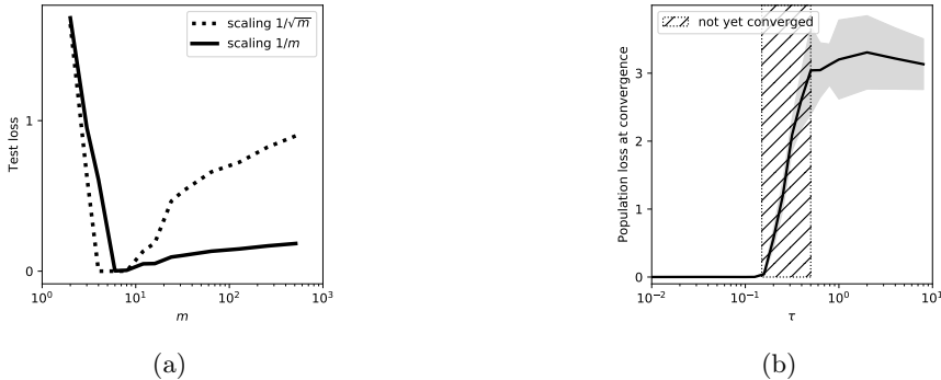
Figure 2: (a) Generalization when \alpha depends on m as \alpha = 1/m or \alpha = 1/\sqrt{m} , the latter leading to lazy training for large m (not symmetrized). (b) Population loss at convergence versus \tau for SGD with a random \mathcal{N}(0, \tau^2) initialization (symmetrized). In the hatched area the loss was still slowly decreasing.
