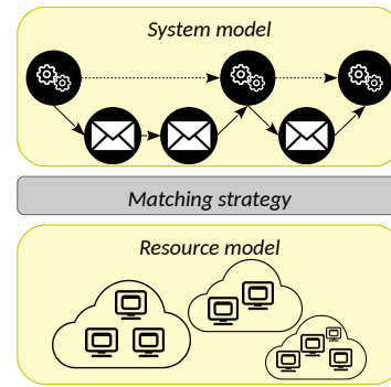
Figure 5: Overall architecture.
