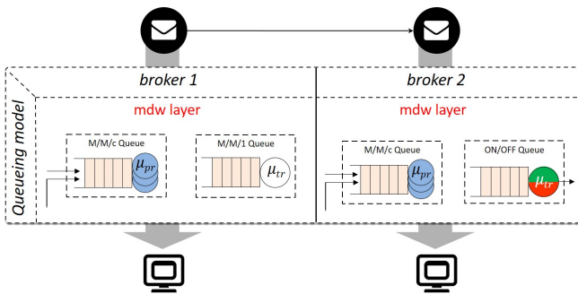
Figure 4: Performance model for the middleware layer in pub/sub systems.
