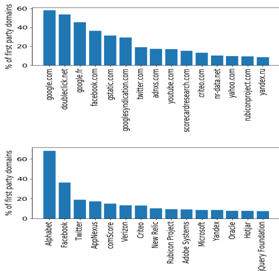
Fig. 5. Basic tracking: Top 15 cross-site trackers and companies included in 8,744 domains.
