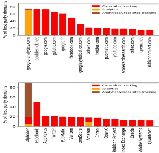
Fig. 4. Top 15 domains and companies involved in analytics, cross-site tracking or both on the same first-party domain.
