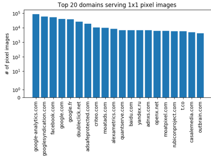
Fig. 13. Top 20 domains responsible for serving invisible pixels
