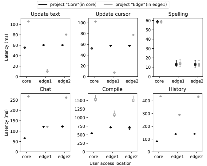
Figure 7: Impact of redirection and user access points.
