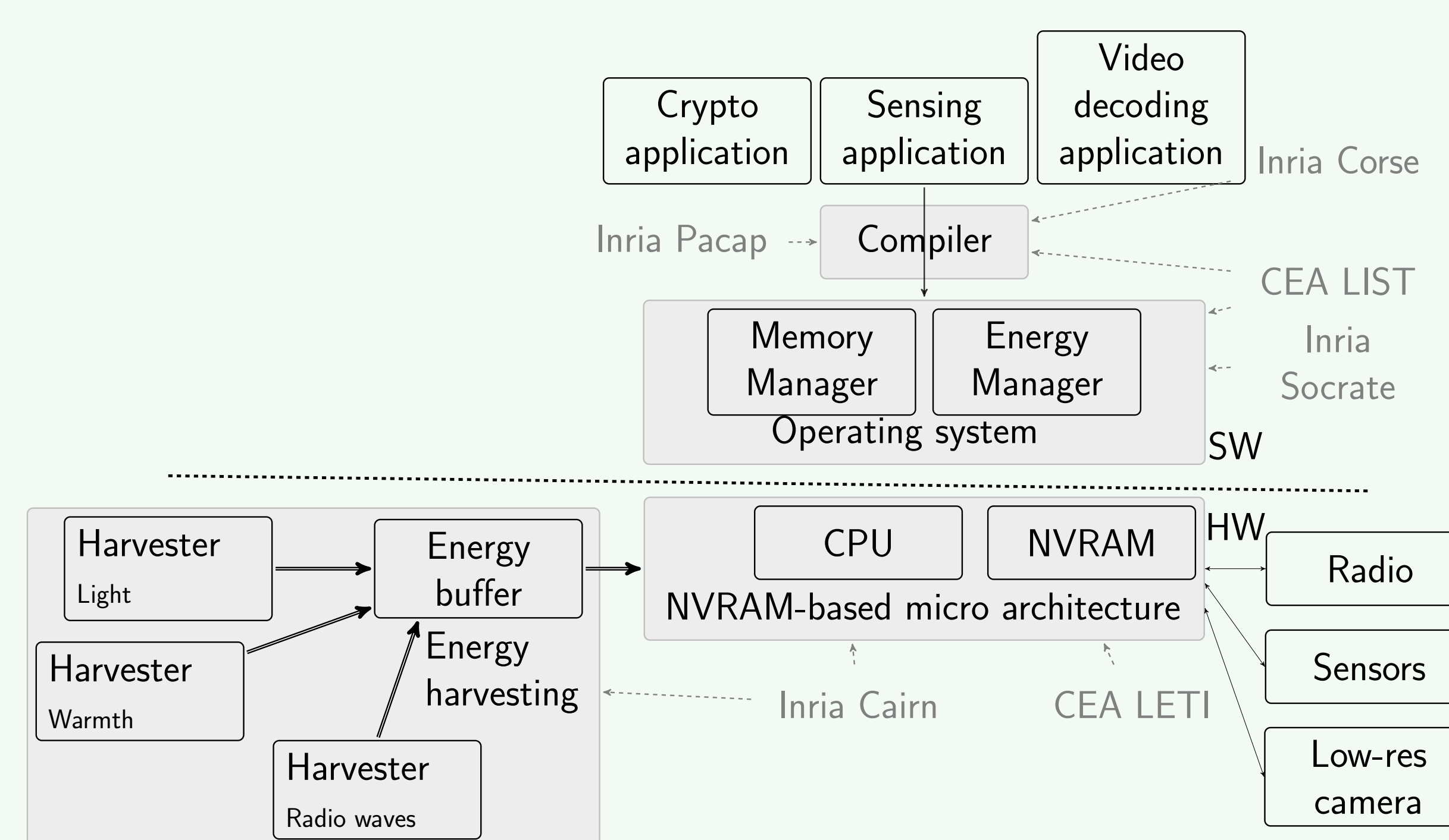
Figure: Overview of the ZEP resulting prototype
