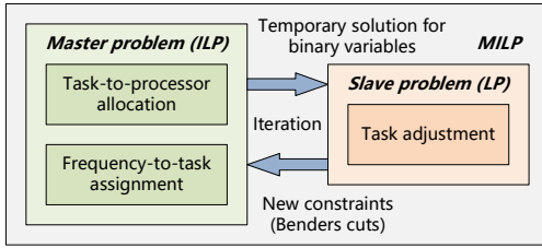
Fig. 1. The structure of OJTM algorithm.
