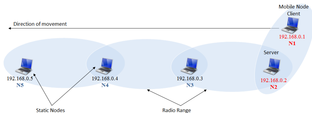
Fig. 8 Chain and wireless links in the testbed.
