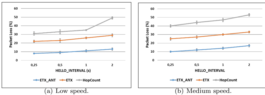
Fig. 9 Packet losses for different HELLO_INTERVAL and two speeds. TC_INTERVAL=2 sec.
