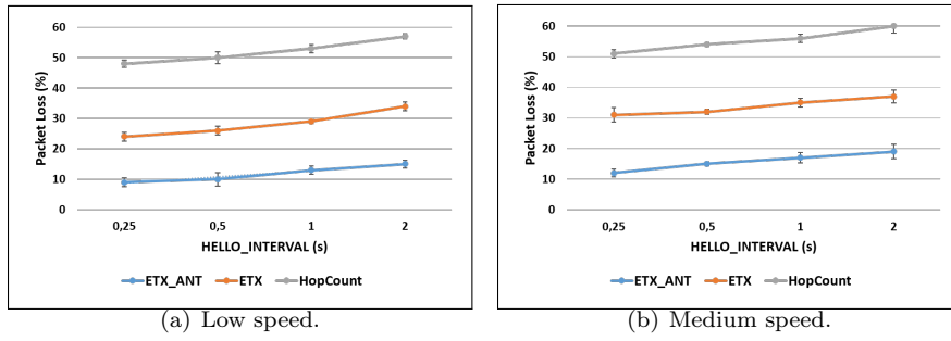
Fig. 10 Packet losses for different HELLO_INTERVAL and two speeds. TC_INTERVAL=5 sec.
