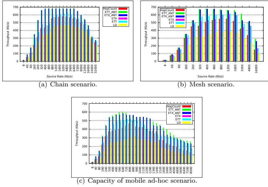
Fig. 5 Throughput for the three scenarios.
