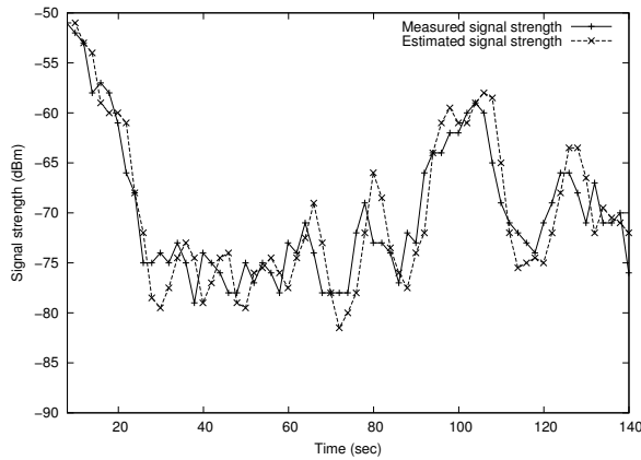
Fig. 1 Comparison of the measured signal strength and the prediction (made 2 seconds in advance).
