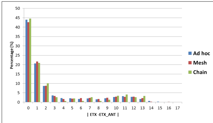
Fig. 3 Distribution of the errors computed as the difference between the anticipated ETX value and the real value: |ETX - ETX_{ANT}| . The speed for the three scenarios is 10\text{km/h} .
