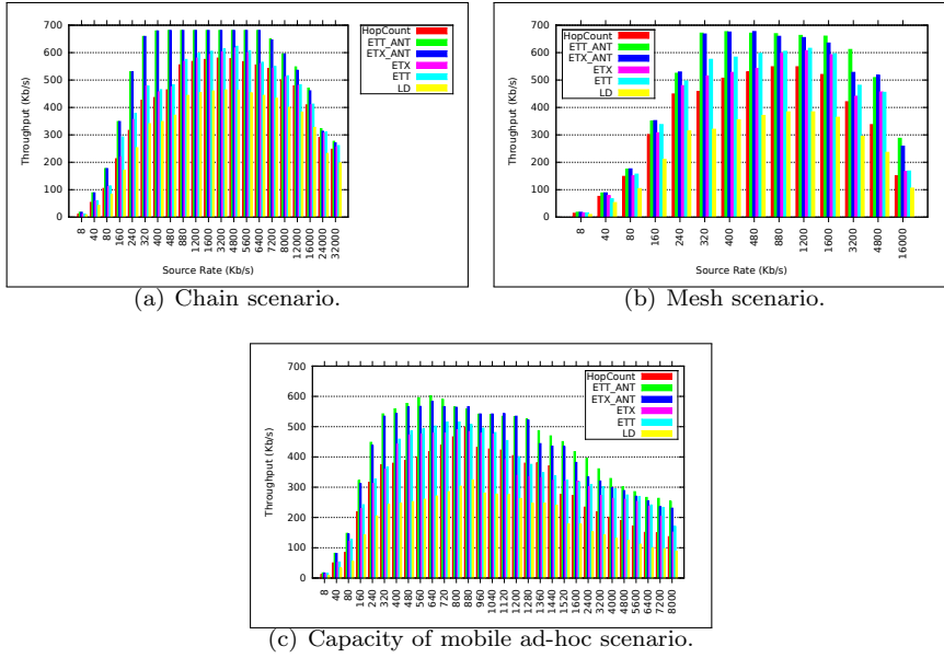
Fig. 5 Throughput for the three scenarios.
