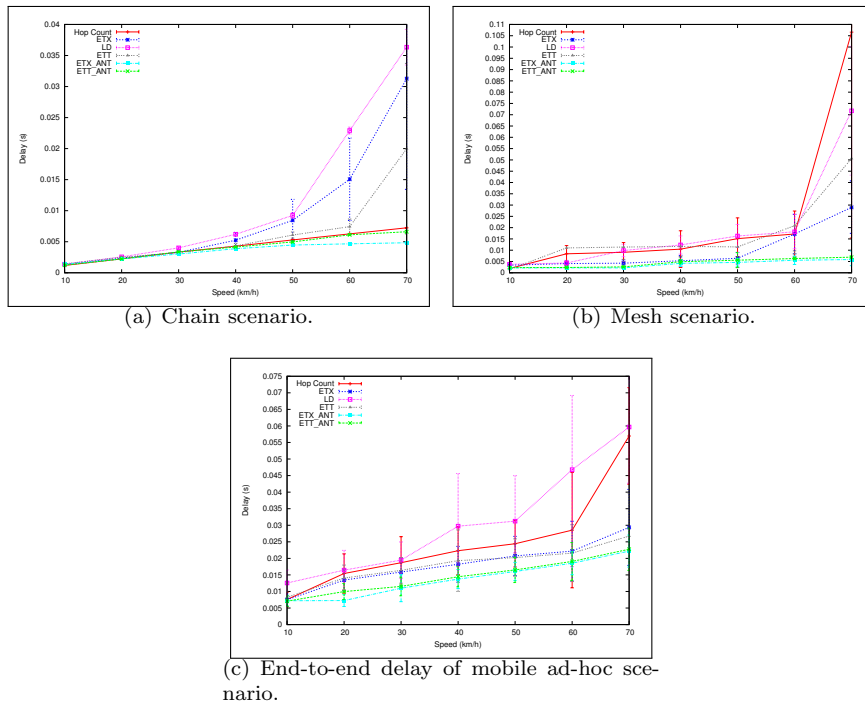
Fig. 6 End-to-end delay for the three scenarios.
