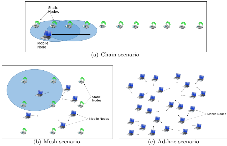
Fig. 2 The three different scenarios. Blue circles represent the radio ranges of the static nodes.
